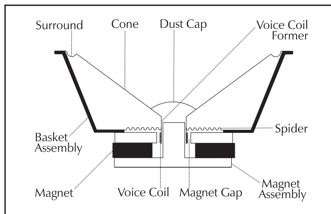
Figure 15. Cut away view of a typical moving coil driver. Notice the complexity due to the high number of parts.
